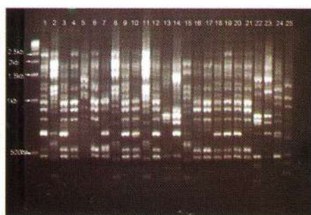
Fig. 22 RAPD of PCR of FOC isolates by primer OPB-07 (Rasthali)
