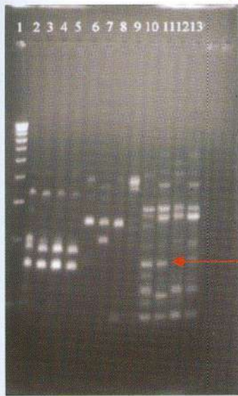
Fig 4. Arrow showing informative bands (777 bp) of OPC-20 primer for resistance cultivars
