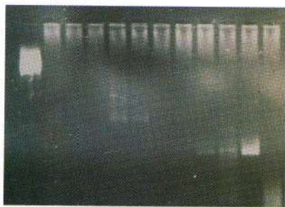
Fig. 20: Detection BSV in M.accuminata spp zebrina
