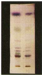
Fig. 12 Separation of banana leafsheath volatiles by Solvent Extraction Method
