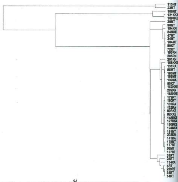
Fig. 23 Phylogram of Foc isolates based on the sequence of rDNA-ITS region
