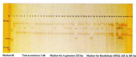
Fig 2. Diversity of ABB germplasm using SSR Markers
