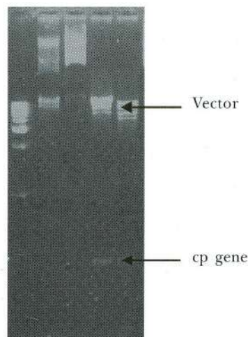
Fig. 29 Restriction digestion analysis of pBinAR having BBTB cp gene
